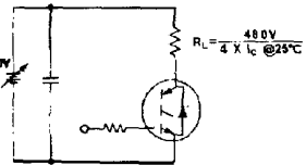
Fig. 20 - Pulsed Collector Current Test Circuit
