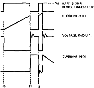
Fig. 18a - Macro Waveforms for Test Circuit of Fig. 18a
