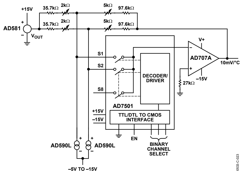
Figure 23. 8-Channel Multiplexer
