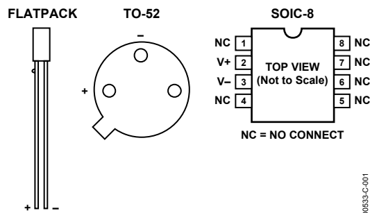
Figure 1. Pin Designations
