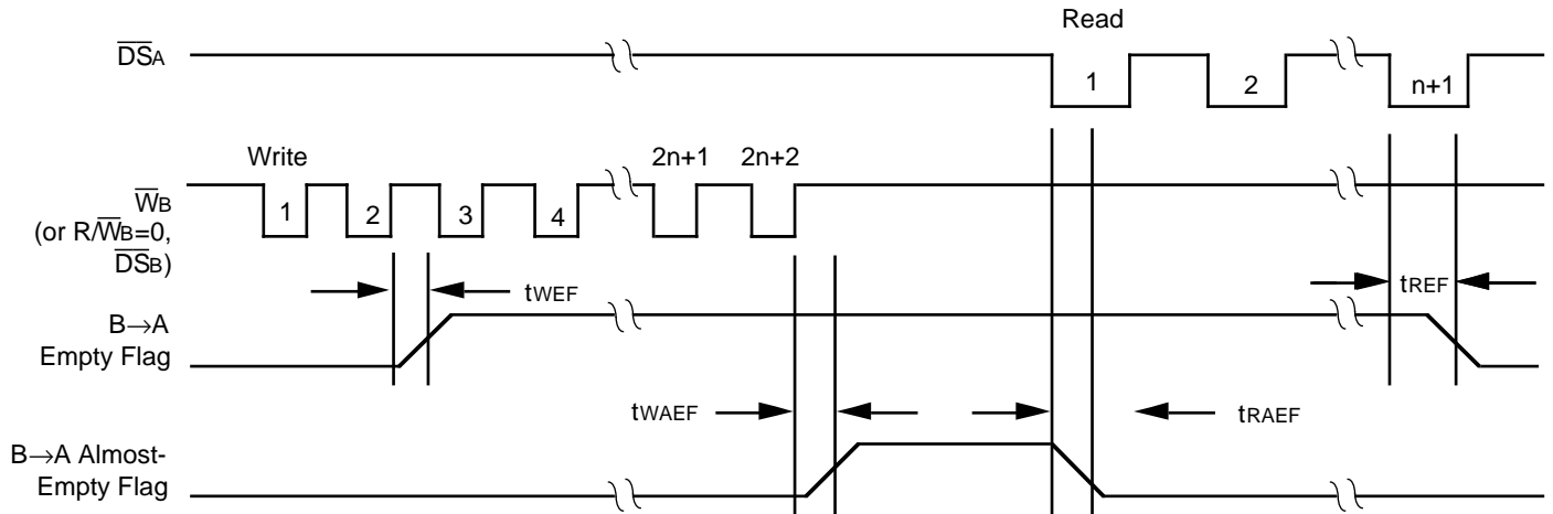
Figure 20. Empty and Almost-Empty Flag Timing for B/A FIFO. (n = Programmed Offset)
