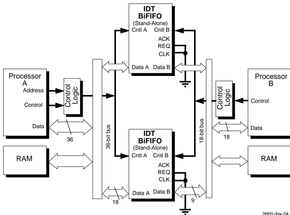
Figure 1. 36- to 18-Bit Processor Interface Configuration
