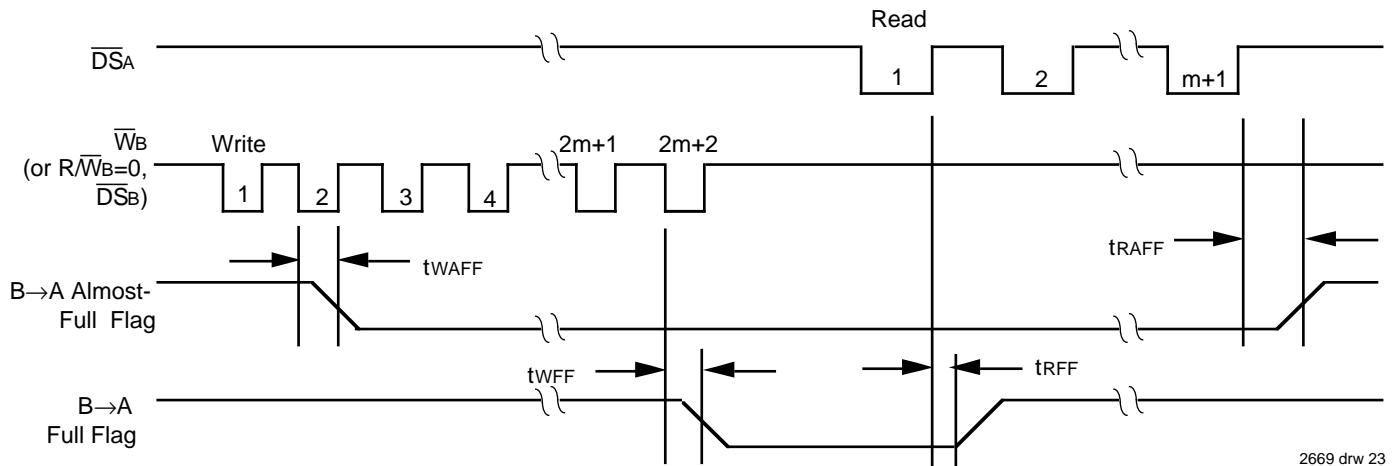
Figure 21. Full and Almost-Full Flag Timing for B/A FIFO. (m = Programmed Offset)
