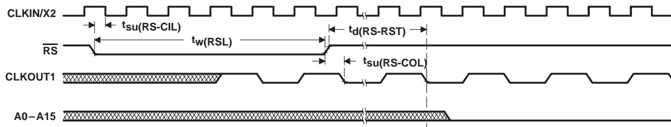
Figure 14. Reset Timing for TMS320C203/LC203
