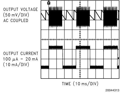
Load Step Response
