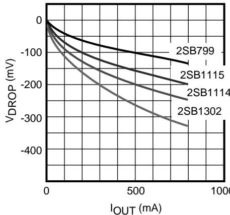
DROPOUT VOLTAGE vs. OUTPUT CURRENT AND EXTERNAL TRANSISTORS
