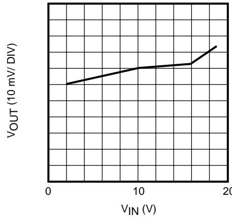
LINE REGULATION 2
