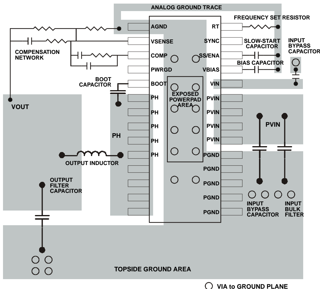
Figure 10. TPS54010 Layout
