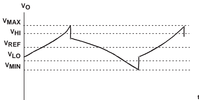
Figure 18. Output Ripple
