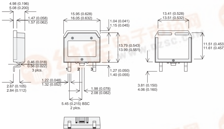
D 3 PAK Package Outline. Dimensions in mm (inches)
