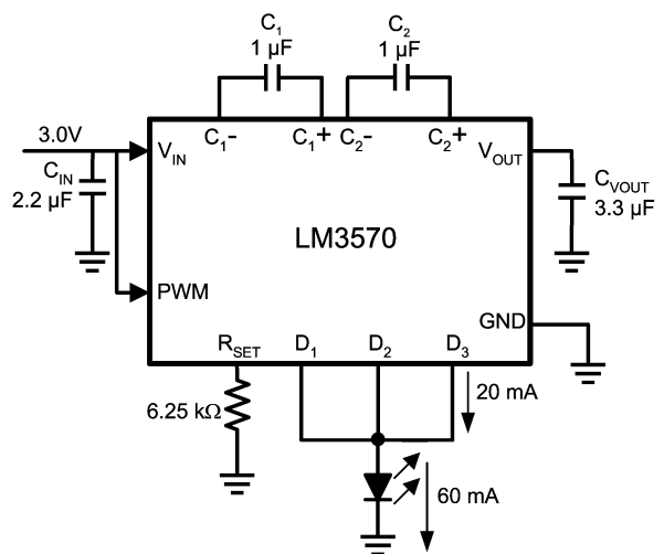
FIGURE 3. One Parallel Connected LED
