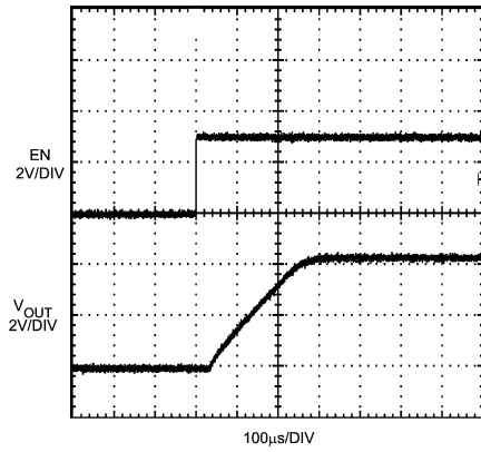
Startup Response
