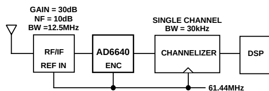
Figure 50. Receiver Analysis
