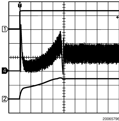
Start-Up: LM3500-21
