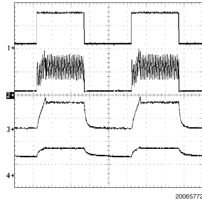
\overline{\text{SHDN}} Pin Duty Cycle Control Waveforms
