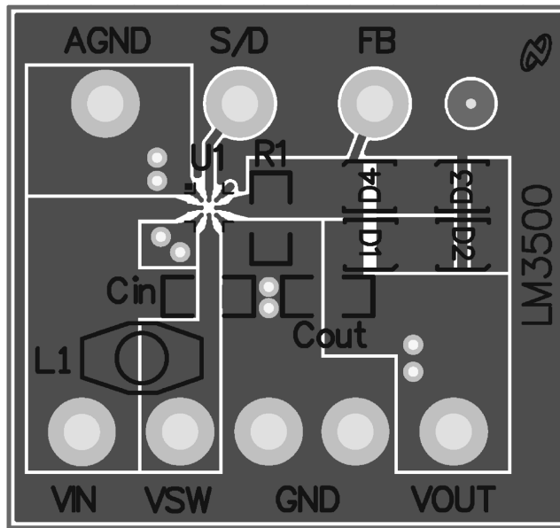
FIGURE 2. Evaluation Board Layout (2X Magnification) Top Layer
