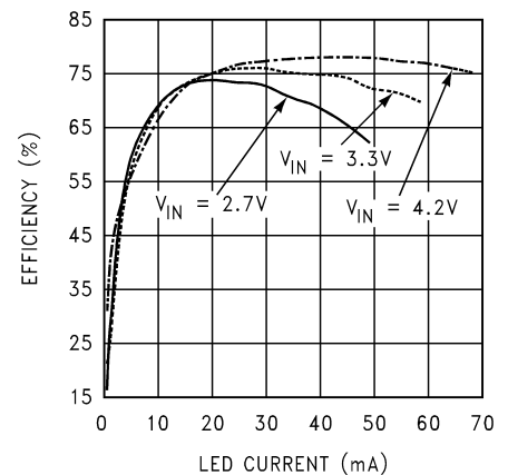
3 LED Efficiency vs LED Current
