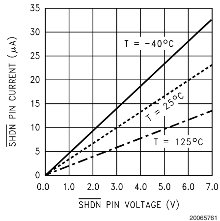
\overline{SHDN} Pin Current vs \overline{SHDN} Pin Voltage
