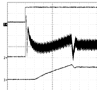
Start-Up: LM3500-16
