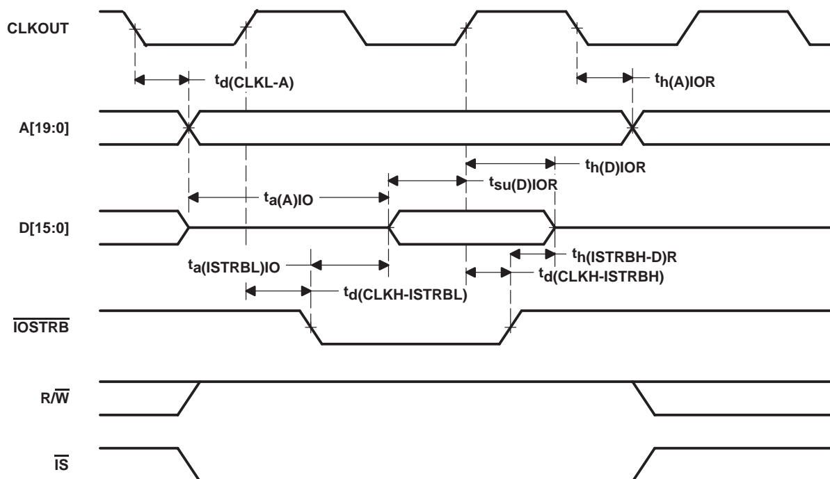
Figure 14. Parallel I/O Port Read ( \overline{\text{IOSTRB}} = 0 )
