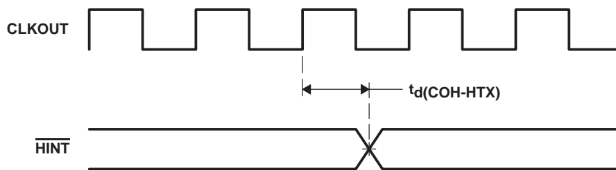
Figure 36. \overline{\text{HINT}} Timing
