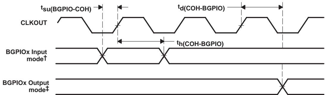
Figure 29. McBSP General-Purpose I/O Timings
