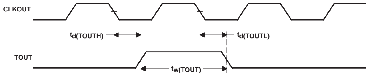
Figure 26. TOUT Timing
