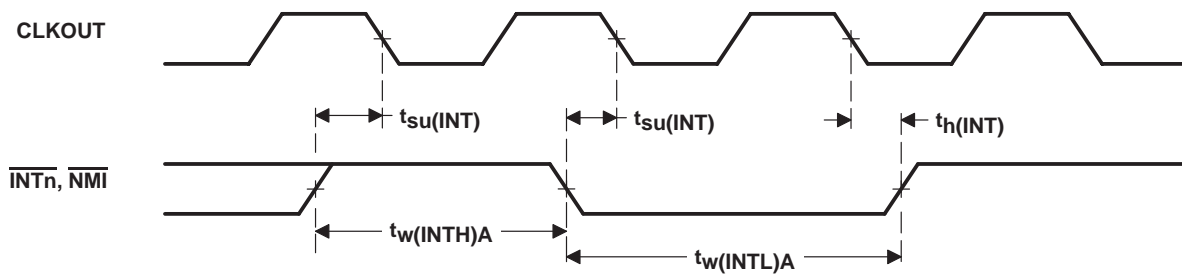
Figure 22. Interrupt Timing
