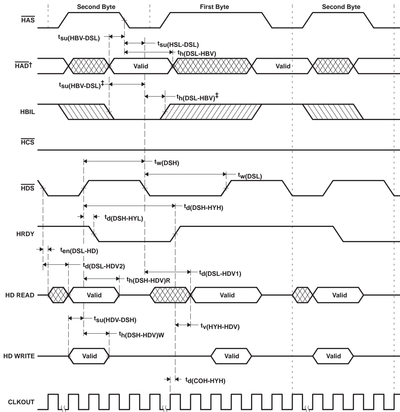
Figure 34. Using \overline{\text{HDS}} to Control Accesses ( \overline{\text{HCS}} Always Low)
