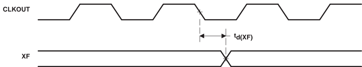
Figure 25. XF Timing
