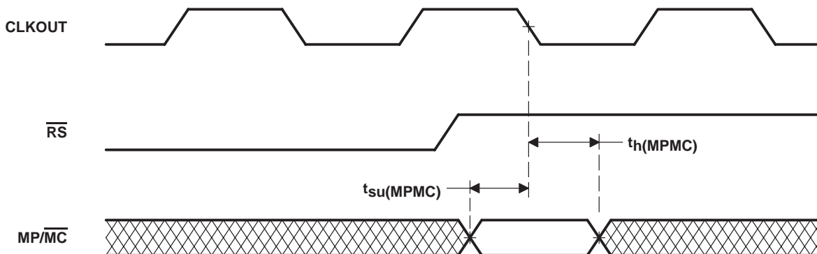
Figure 23. \text{MP}/\overline{\text{MC}} Timing
