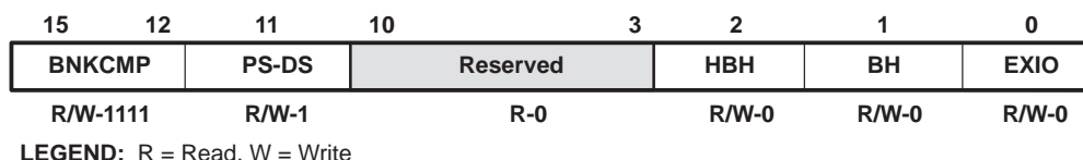
Figure 5. Bank-Switching Control Register (BSCR) [MMR Address 0029h]
