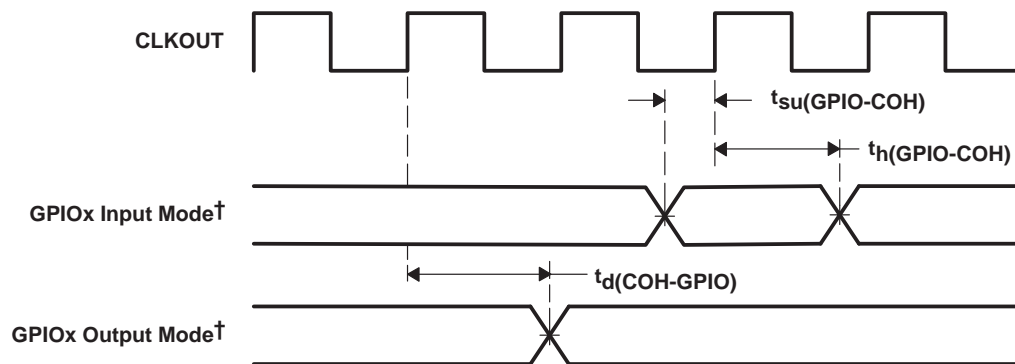
Figure 37. GPIOx ^\dagger Timings
