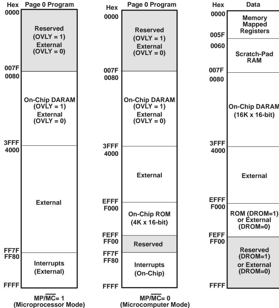
Figure 1. Memory Map
