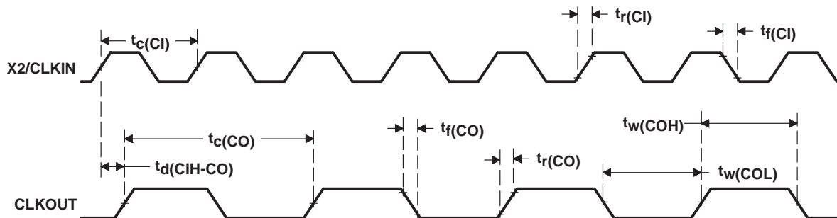
Figure 10. External Divide-by-Two Clock Timing
