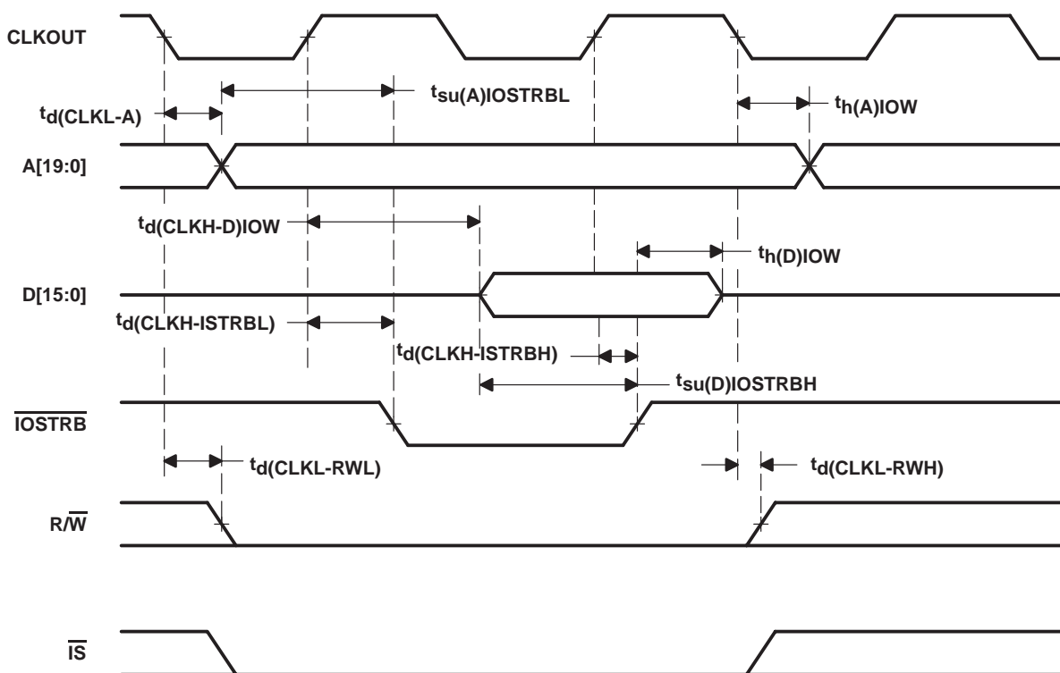
Figure 15. Parallel I/O Port Write ( \overline{\text{IOSTRB}} = 0 )
