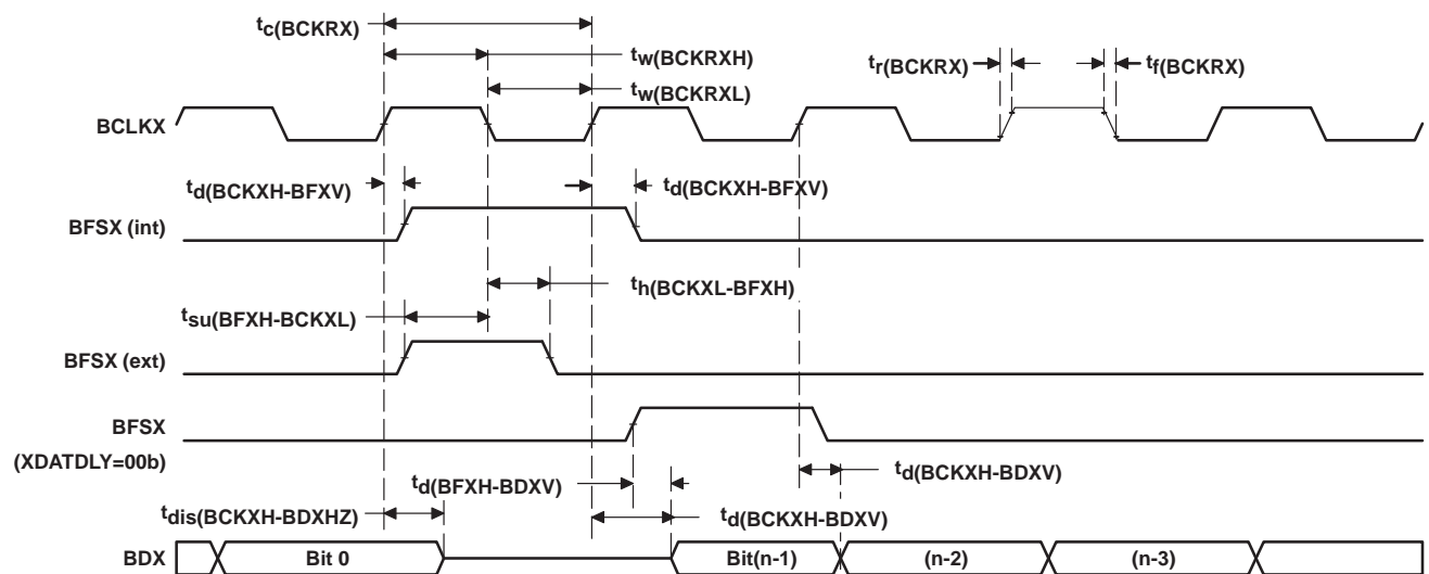
Figure 28. McBSP Transmit Timings
