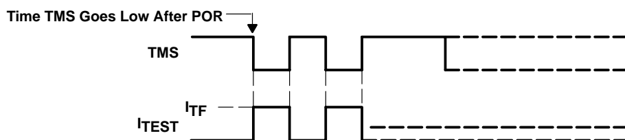
Figure 13. Fuse Check Mode Current, MSP430F12x
