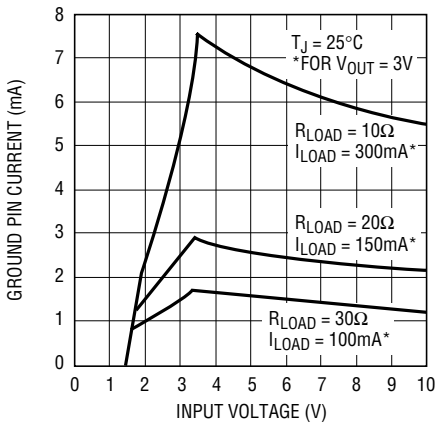
LT1521-3 Ground Pin Current
