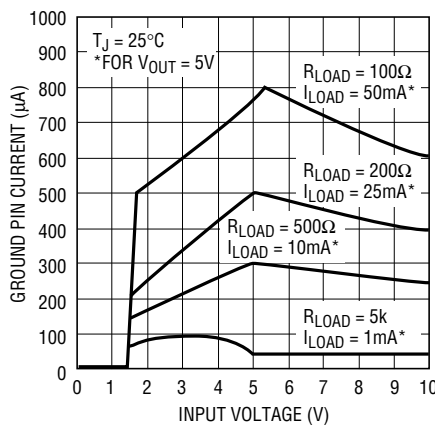
LT1521-5 Ground Pin Current
