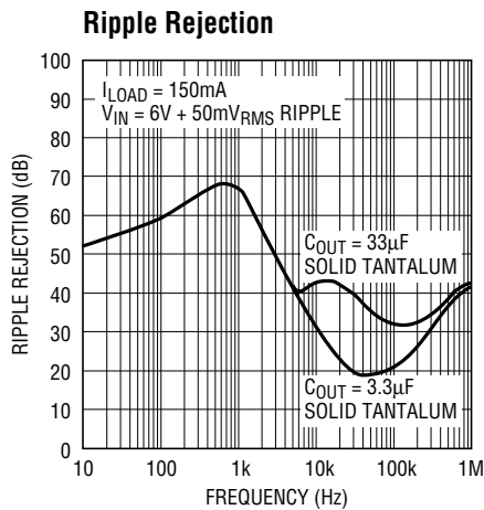
LT1521 • TPC31
