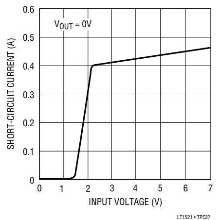
Current Limit
