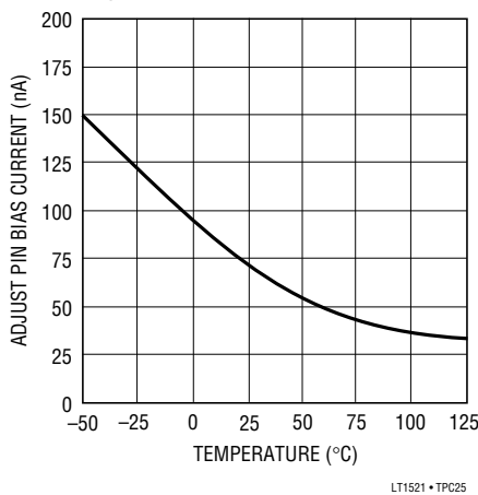
Adjust Pin Bias Current
