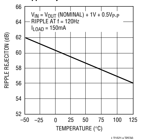
Ripple Rejection
