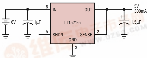
5V Battery-Powered Supply with Shutdown
