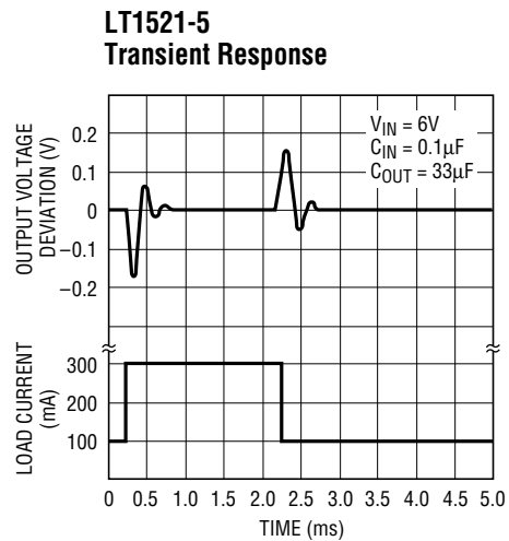
LT1521 • TPC34
