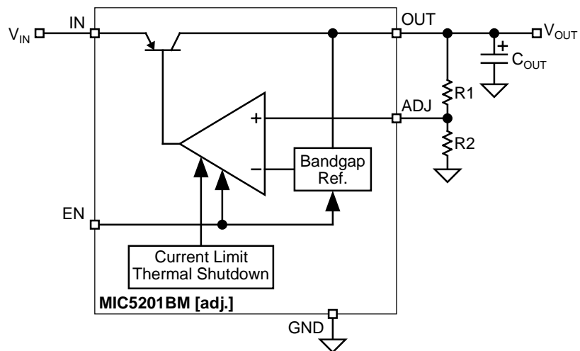
Adjustable Regulator
