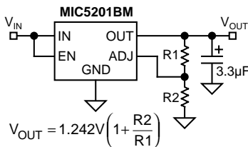
Figure 2. Adjustable Application
