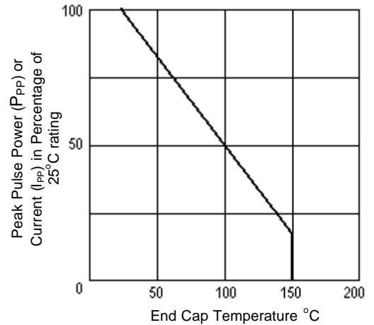
FIGURE 2 Derating Curve
