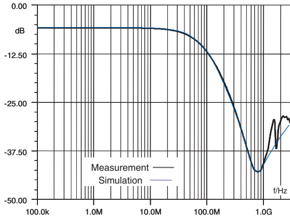
Fig. 3: Digital crosstalk measurements.
