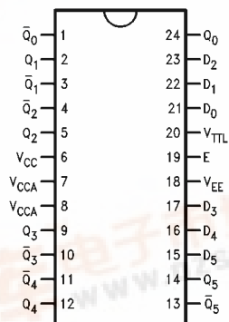
24-Pin DIP/SOIC
