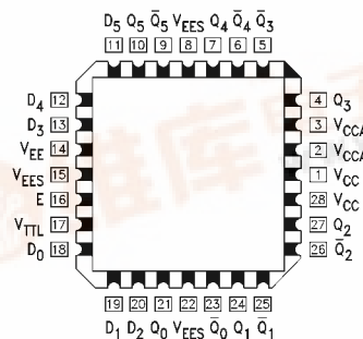
28-Pin PLCC
