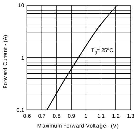
Fig. 2 - Forward Characteristic
