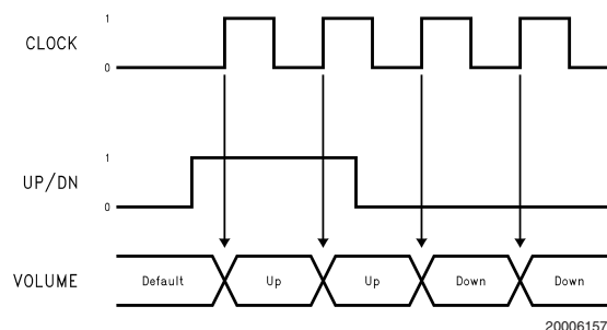
FIGURE 2. Timing Diagram
