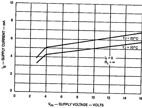
H11V SUPPLY CURRENT vs. SUPPLY VOLTAGE
