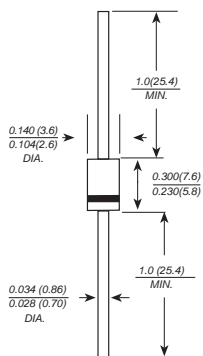
Dimensions in inches and (millimeters)
