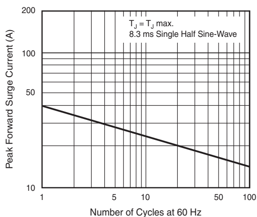
Fig. 6 - Maximum Non-Repetitive Peak Forward Surge Current Uni-Directional Use Only
