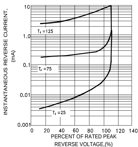
FIG.4-TYPICAL REVERSE CHARACTERISTICS
