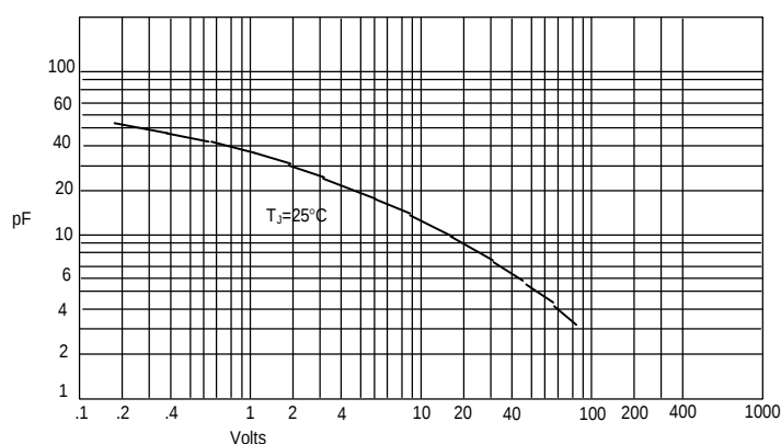
Figure 2 Junction Capacitance
