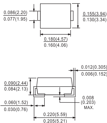
DO-214AA(SMB)
