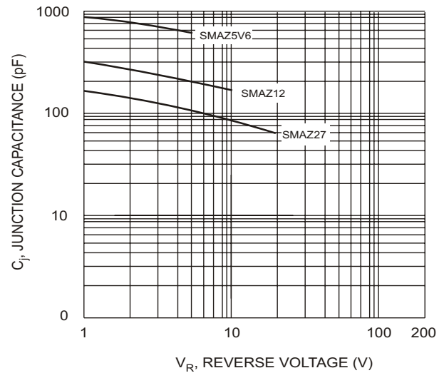
Fig. 2 Junction Capacitance vs Reverse Voltage
