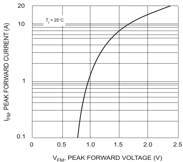
Fig. 3 Peak Forward Current vs Peak Forward Voltage
