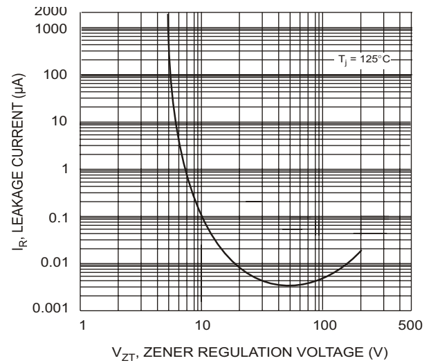
Fig. 4 Leakage Current vs Regulation Voltage
