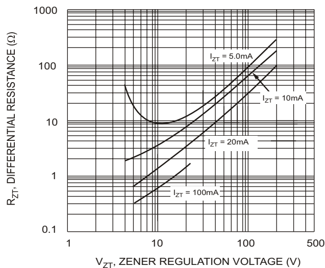
Fig. 5 Differential Resistance vs Regulation Voltage
