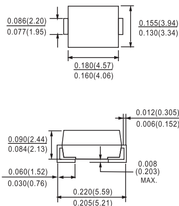
DO-214AA(SMB)
