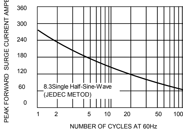
FIG.2-MAXIMUM NON-REPETITIVE SURGE
