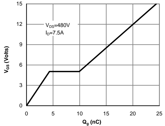
Figure 8: Gate-Charge Characteristics
