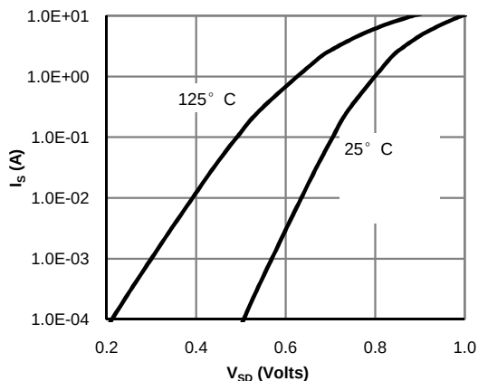
Figure 6: Body-Diode Characteristics
