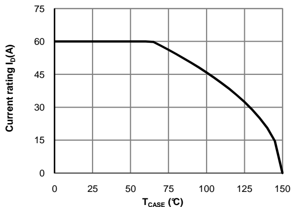
Figure 9: Current De-rating (Note B)
