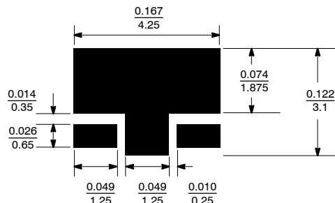
FIGURE 1. Recommended Copper Spreading Footprint
