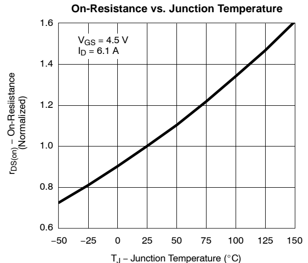
FIGURE 4. Si3434DV
