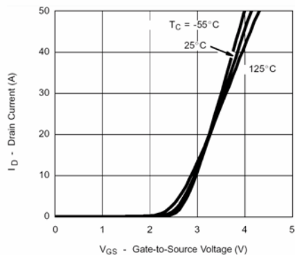
Figure 5. Transfer Characteristics
