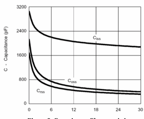
Figure 8. Capacitance Characteristics
