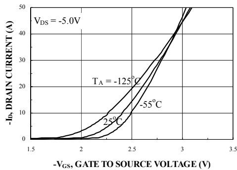
Figure 5. Transfer Characteristics
