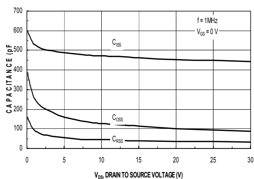
Figure 4. Capacitance Characteristics
