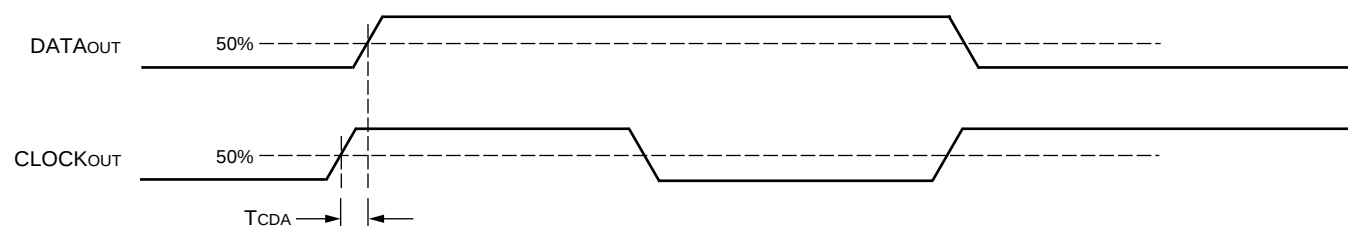
Figure 4. Clock/Data Alignment
