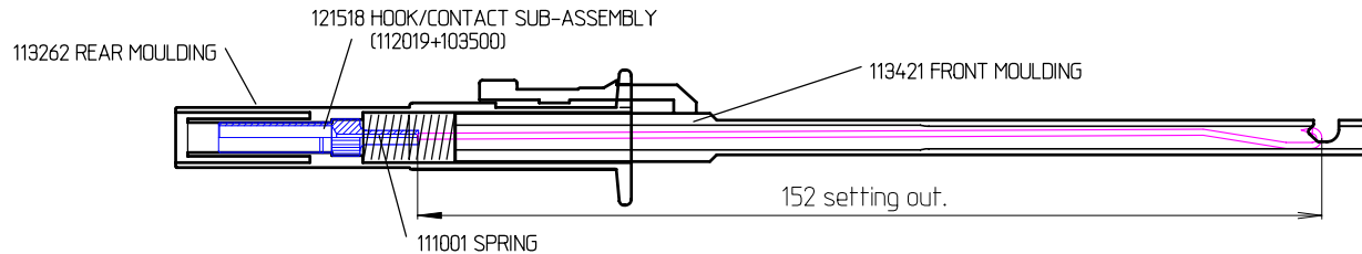
PLAN VIEW
