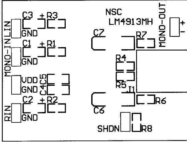
FIGURE 5. Top Overlay
