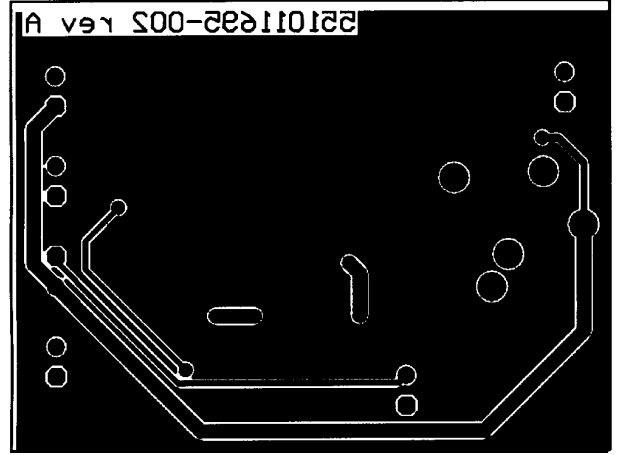
FIGURE 7. Bottom Layer
