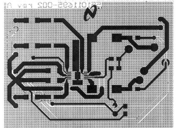
FIGURE 8. Composite Layer
