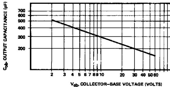
OUTPUT CAPACITANCE vs COLLECTOR BASE VOLTAGE
