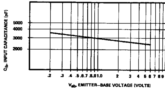
INPUT CAPACITANCE vs EMITTER BASE VOLTAGE
