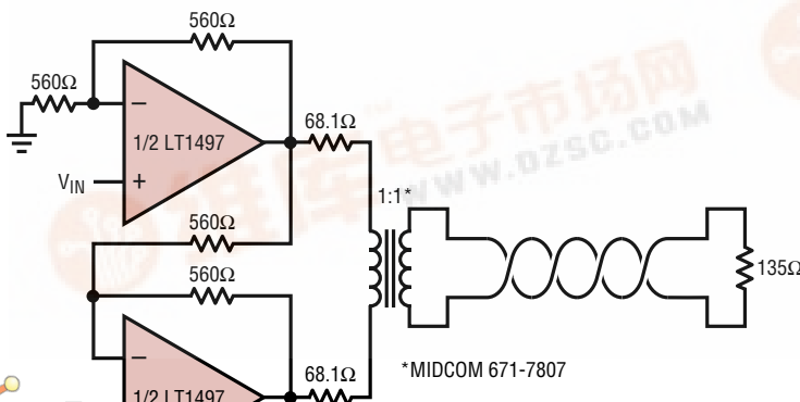
HDSL2 Single Pair Line Driver
