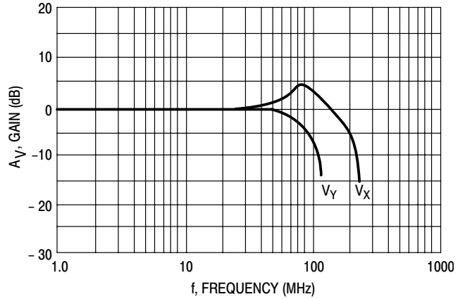
Figure 2. Transconductance Bandwidth
