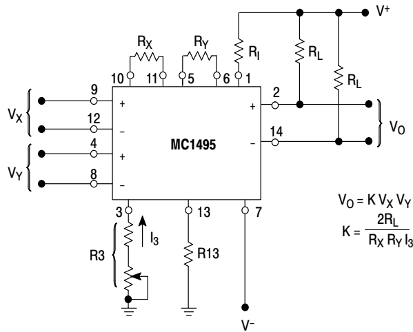
Figure 20. Basic Multiplier
