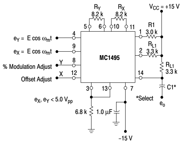
Figure 30. Amplitude Modulation
