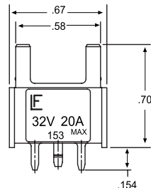
Single or stackable end unit (Part No. 01530032)
