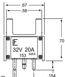
Stackable unit (Part No. 01530033)
