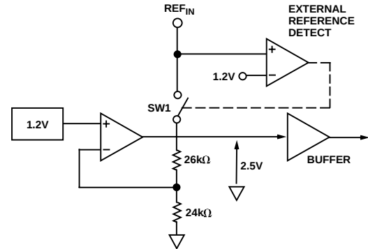
Figure 9. On-Chip Reference
