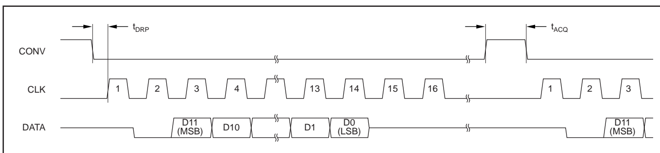
FIGURE 9. Typical SPI/QSPI Interface Timing.
