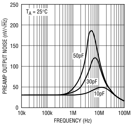
Preamp Output Noise vs Input Capacitance
