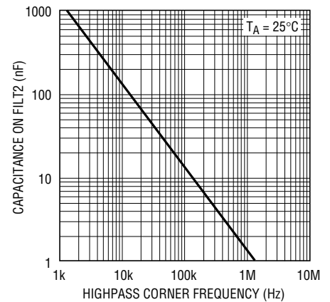
Gain Stage Highpass vs Capacitance on FILT2 or FILT2L
