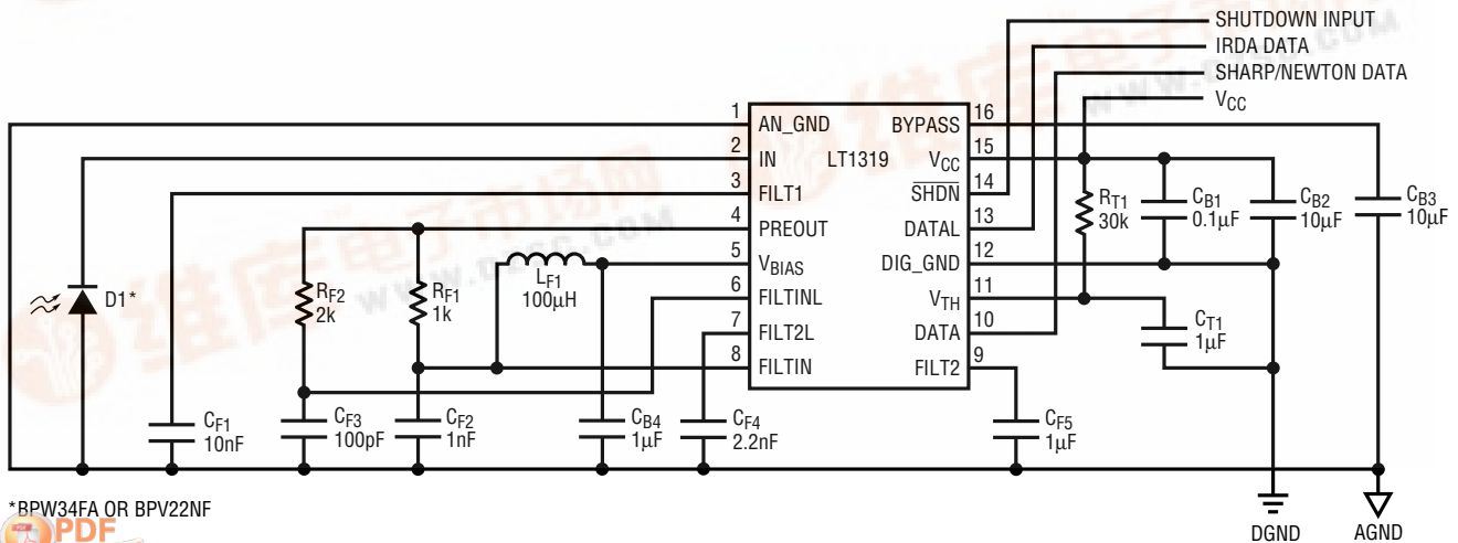
IRDA and Sharp/Newton Data Receiver
