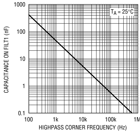
Preamp Highpass vs Capacitance on FILT1
