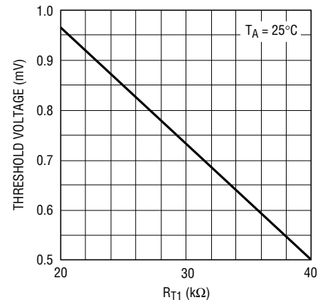
FILTIN- or FILTINL- Referred Threshold Voltage vs R T1
