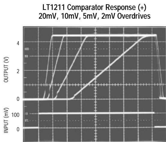
V_S = 5V R_L = \infty 5µs/DIV 1211/12 AI01
