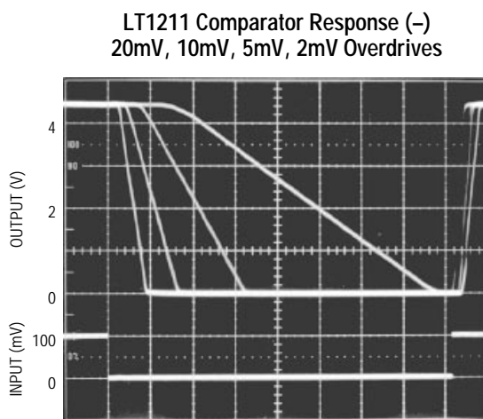
V_S = 5V R_L = \infty 5µs/DIV 1211/12 AI02
