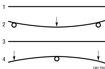
Figure 4. Flexure Numbers
